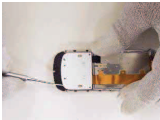
22) Use the dental pick to release the UI Flex.
