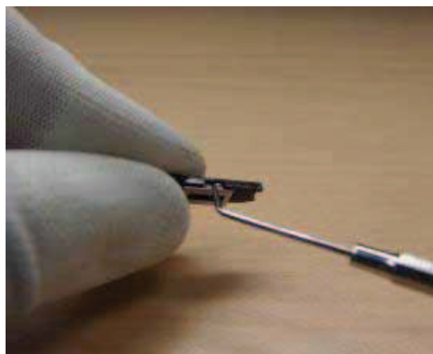
12) Use the dental pick to release the earpiece from the frame.
