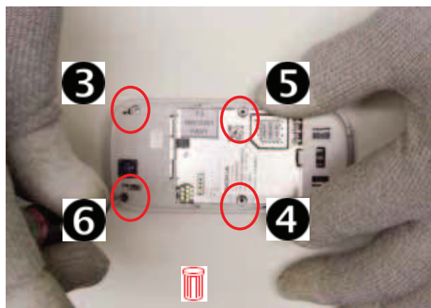
8) Use the #6 TORX screwdriver to remove the 4 screws in the order shown. Discard the screws.
